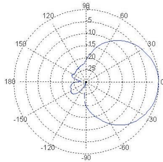
Elevation (E-field) radiation pattern
